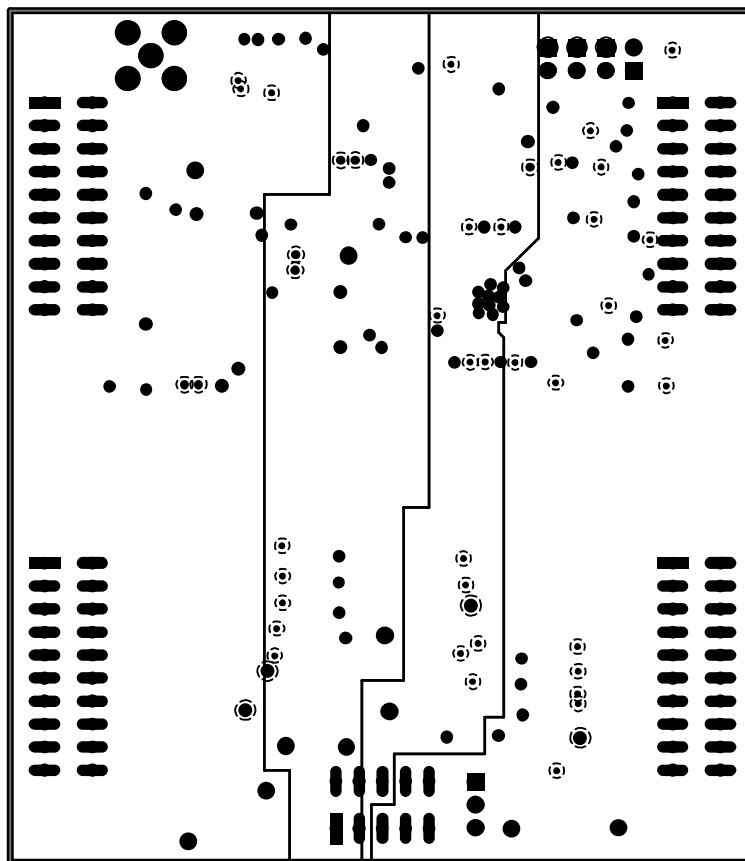
Figure 3. Power Plane
